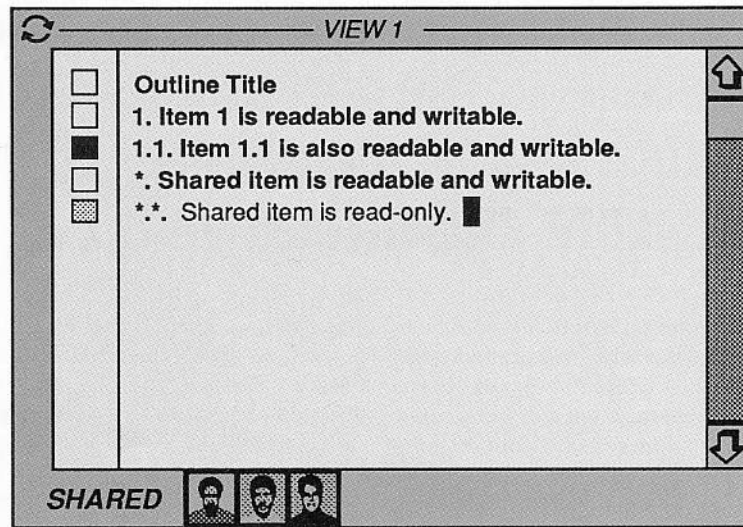
FIGURE 3. A GROVE Group Window.
